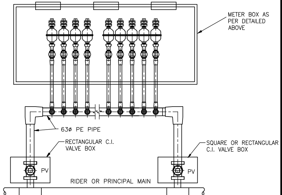
RING ARRANGEMENT FOR THIRTEEN TO TWENTY METERS
