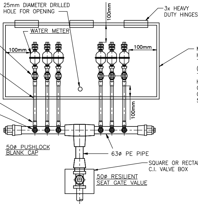
MANIFOLD ASSEMBLY FOR SIX TO TWELVE WATER CONNECTIONS
