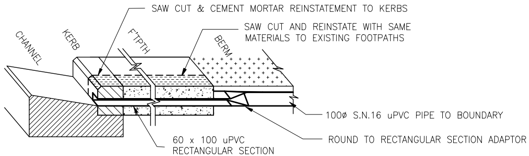
TYPICAL SECTION - KERB OUTLET DETAIL
