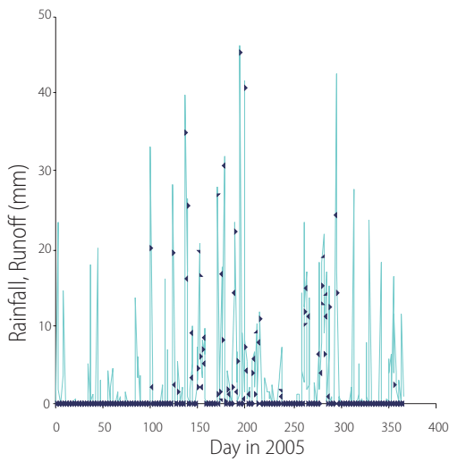
Fig. 3 Modelled storm-water runoff from the 150 mm deep Waitakere Civic Centre greenroof that stores 24 mm of plant-available moisture. The pale blue line shows the rainfall on each day from 1 January to 30 December 2005. The dark blue dots show how much of the rainfall would have seeped from the roof. The model shows this non-irrigated, extensive greenroof would have captured 680 mm of the 1300 mm of rainfall in 2005, including nearly all the rainfall between November and March.
