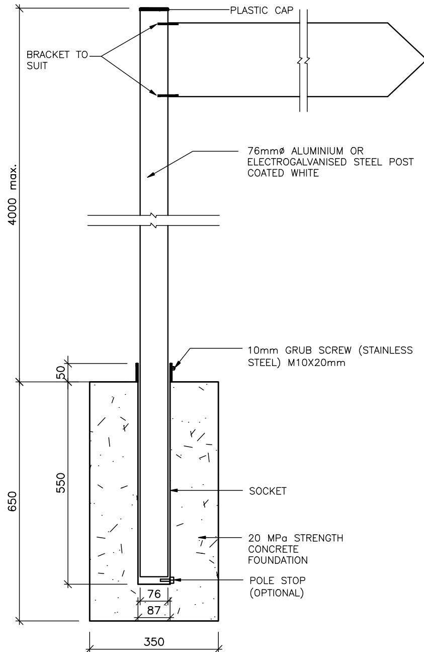
TYPICAL DETAIL SCALE 1:10
