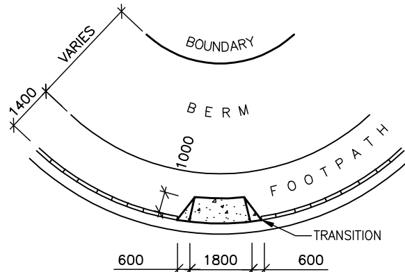
LIPLESS PRAM CROSSING (WHERE FOOTPATH NEXT TO KERB) N.T.S.
