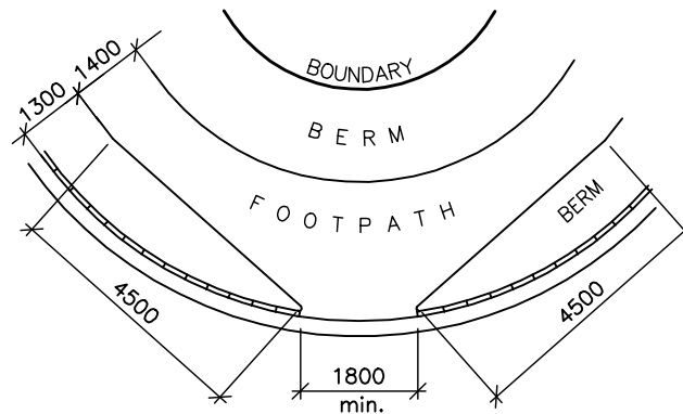
LIPLESS PRAM CROSSING (WHERE FOOTPATH SEPARATED FROM KERB) N.T.S.
