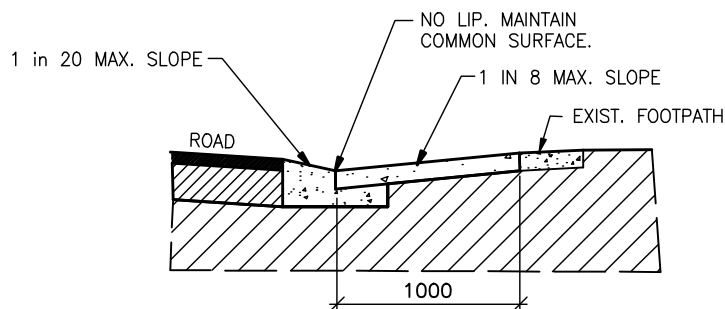
SECTION THROUGH LIPLESS PRAM CROSSING N.T.S.
