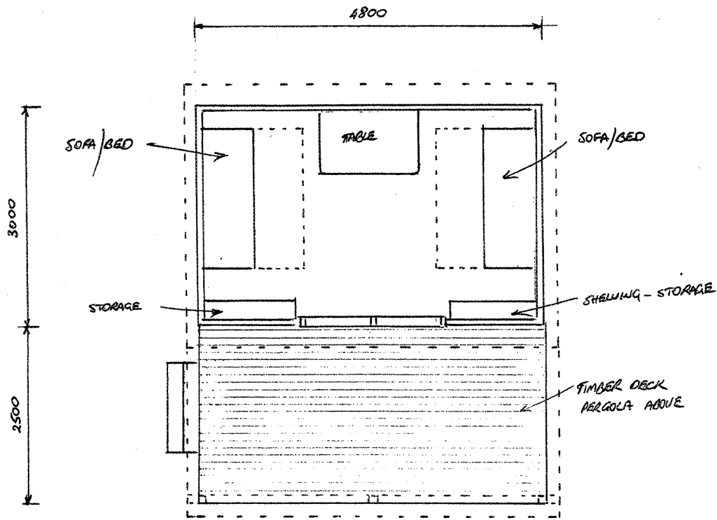
FLOOR PLAN
