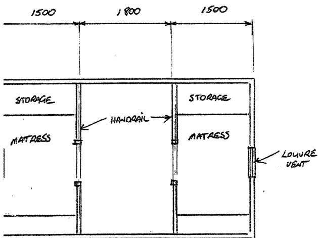
MEZZANINE PLAN
