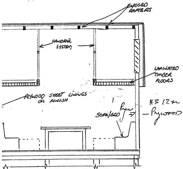
CROSS SECTION
